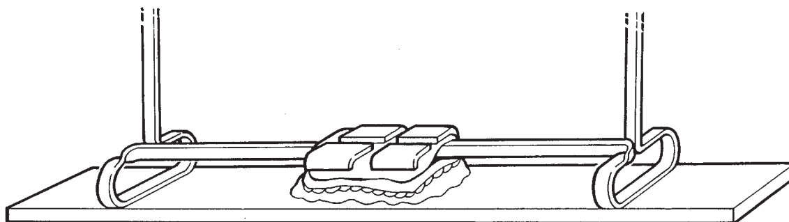
Figure 5 Diagram of the 0.021 \times 0.025 -inch stainless steel wire jig used to support the brackets whilst the adhesive hardened to the steel.
